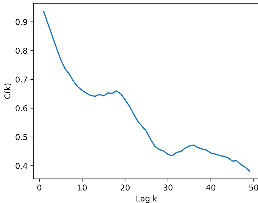
LUMO Autocorrelation
